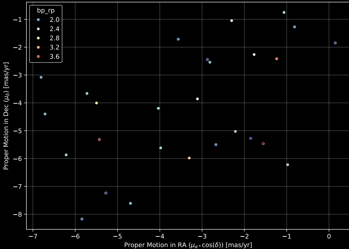
APOGEE DR17 Field: [331+00] Proper Motion Diagram (n= 27)
