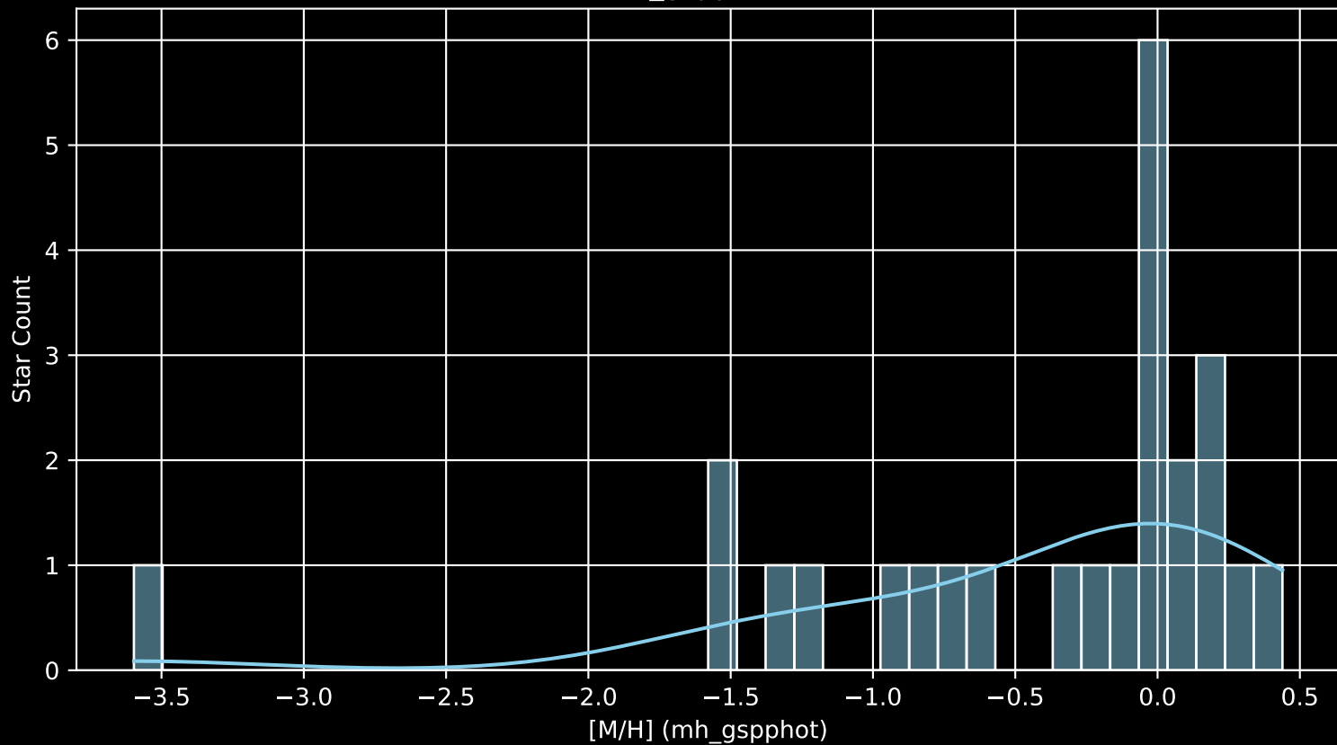
APOGEE DR17 Field: [331+00 [M/H] (mh_gspphot) (n= 25)
