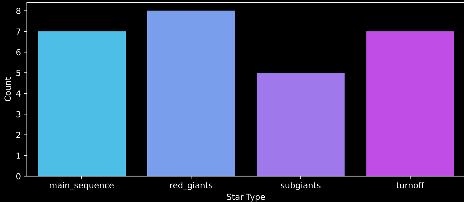
APOGEE DR17 Field: [331+00] Count plot of Star Type
