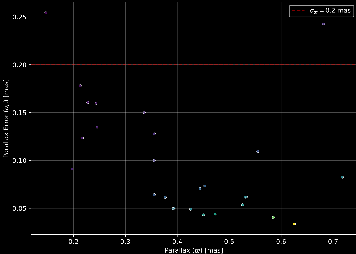
APOGEE DR17 Field: [331+00] Parallax Quality (n= 27)
