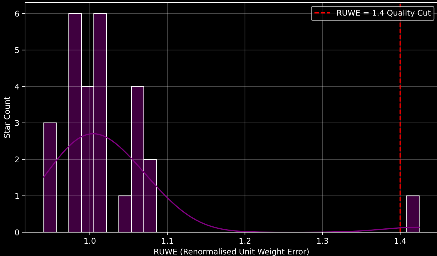
GAPOGEE DR17 Field [331+00] RUWE Distribution (n= 27)
